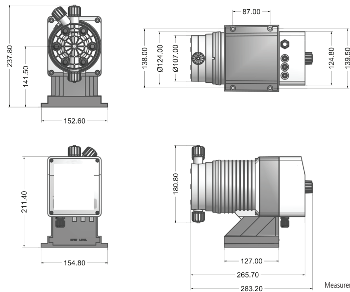
"N" - "P" PUMP HEAD
